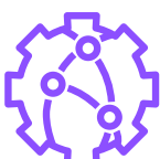
CloudFront Functions
