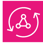
AppSync
