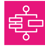
Step Functions
