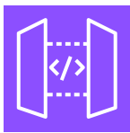
Api Gateway
